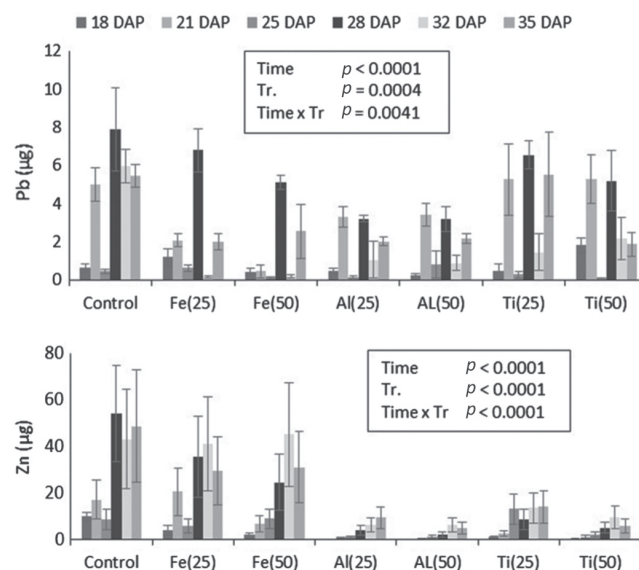
Fig. 2. Leachate metal contents in contaminated soil (control) and soil amended with nano-oxides of Fe, Al, and Ti at rates of 25 g.kg -1 (25) and 50 g.kg -1 (50), collected at 18, 21, 25, 28, 32, 35 d after plant emergence (DAP). The vertical bars indicate the standard error.
